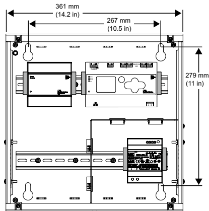
DIN14-P-ACP/SPS Front
