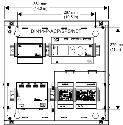
DIN14-P-ACP/SPS/NET Front
