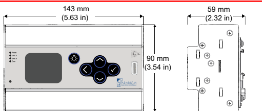
P-ACP-D Front
