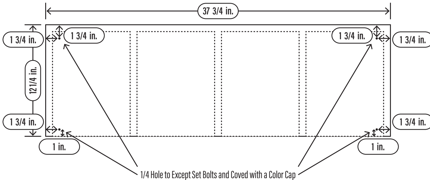
TOP AND BOTTOM VIEW
